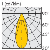
MR16, 6 Вт 58°
