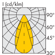
MR16, 6 Вт 70°
